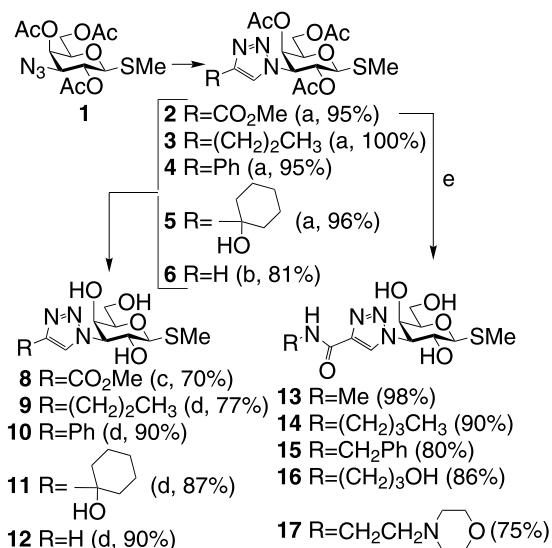
Scheme 1. Reagents and conditions: (a) Cu(I), DIPEA, toluene, 40 °C; (b) Propiolic acid, toluene, 80 °C; (c) NaOMe/MeOH; (d) MeNH_2 40% in H_2O ; (e) RNH_2 , MeOH.
